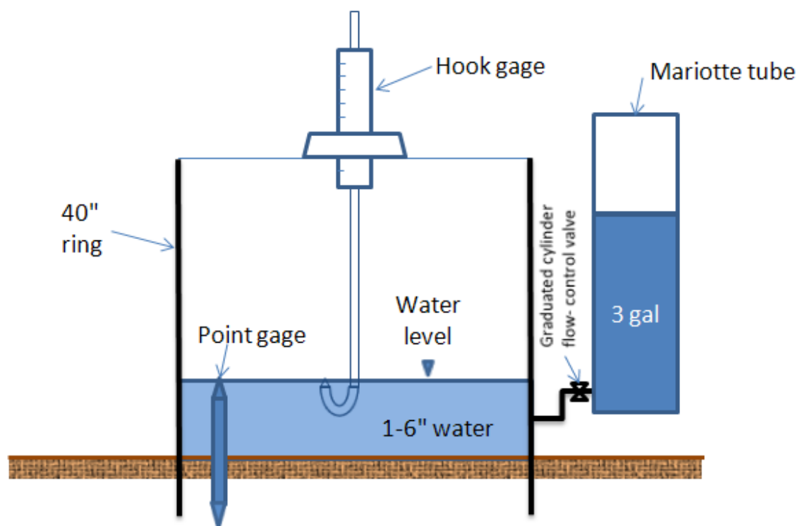
Figure VII.3. Single Ring Infiltrrometer Setup with Mariotte Tube
