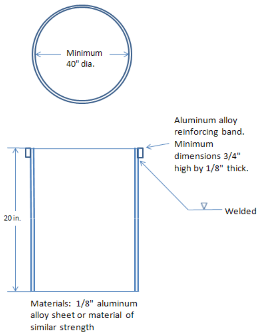
Figure VII.2. Single Ring Infiltrrometer Construction
