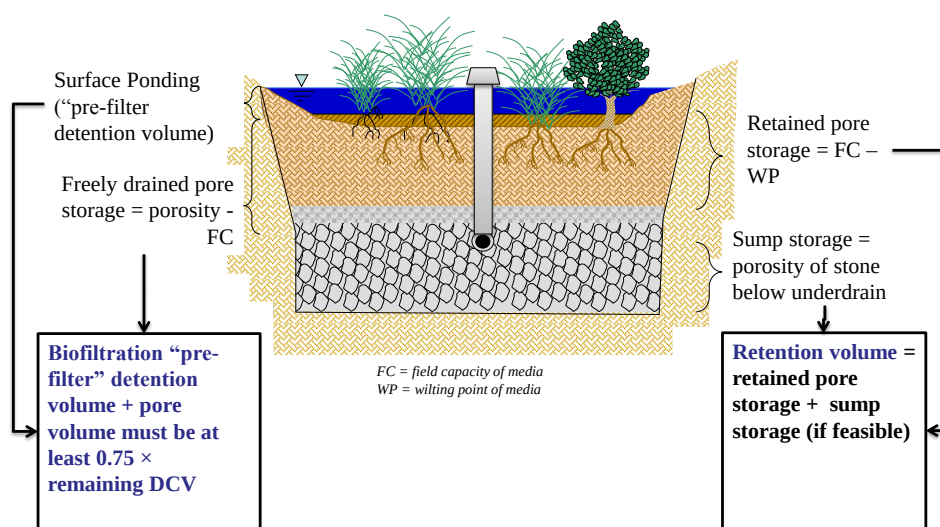
Figure SOC-1. Schematic of Biofiltration Storage Compartments
