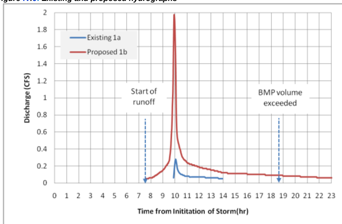
Figure IV.9: Existing and proposed hydrographs
